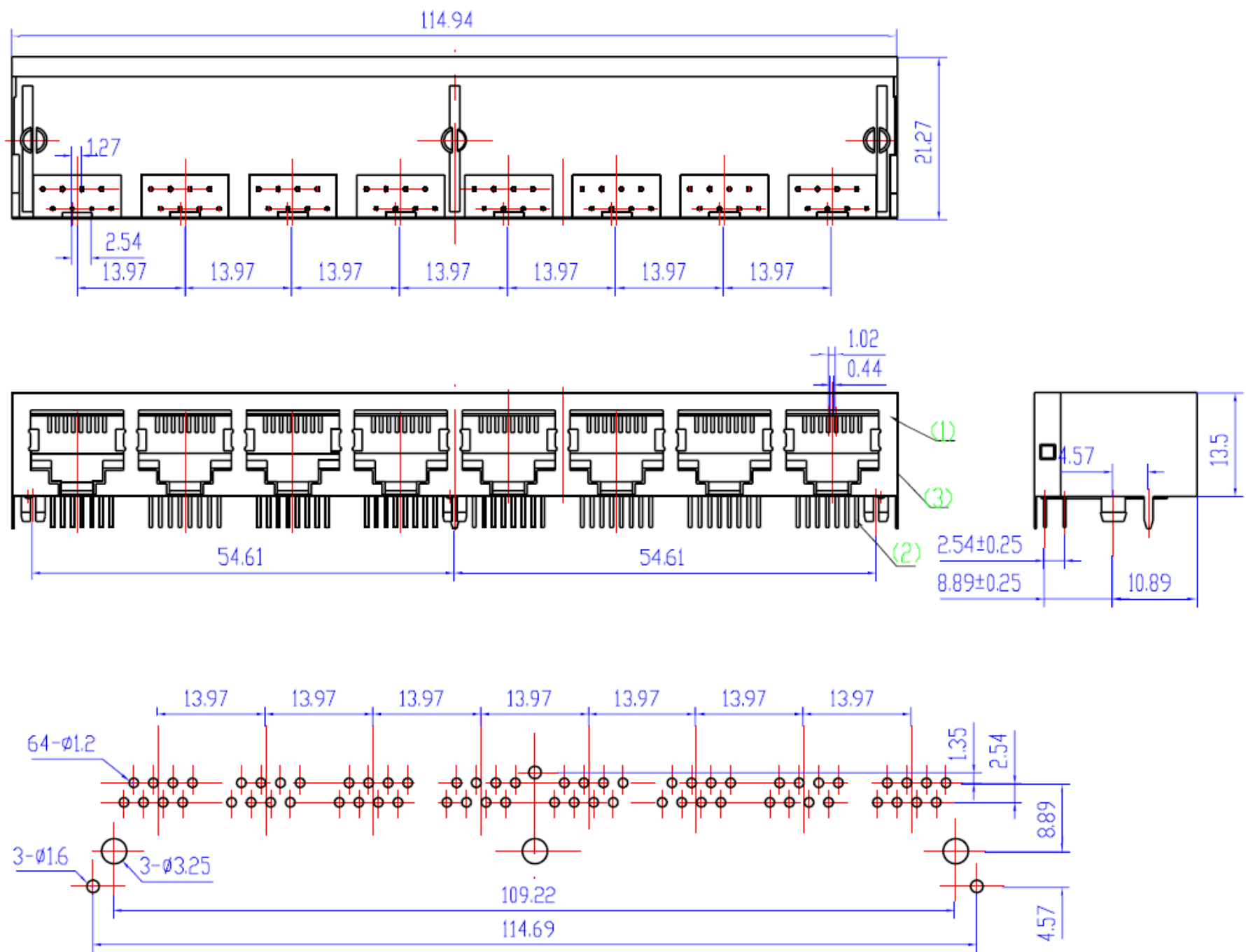
PRAN ELECTRONICS PVT. LTD. RJ45 8 PORT SHIELDED JACK, PART CODE: JP-S1-8P8C-8P-S
