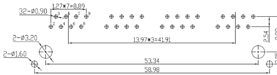
PC Board Layout
