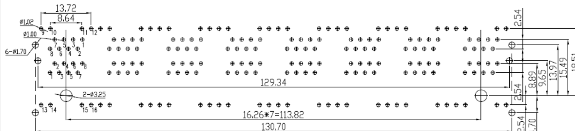
PC Board Layout
